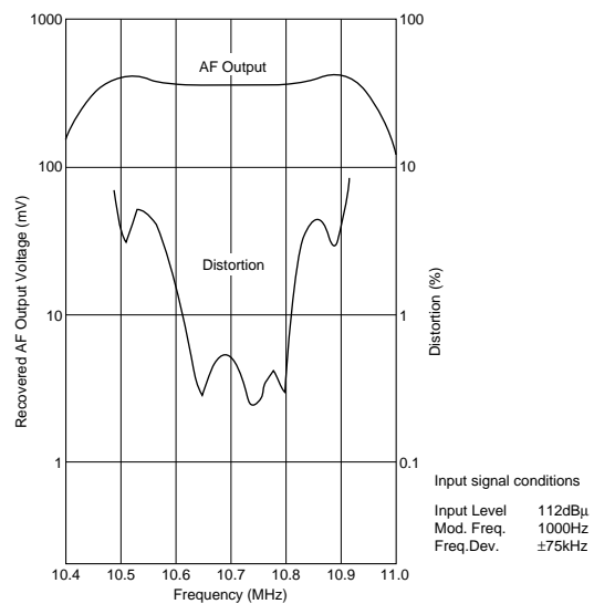
Frequency Characteristics
