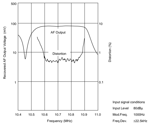
Frequency Characteristics
