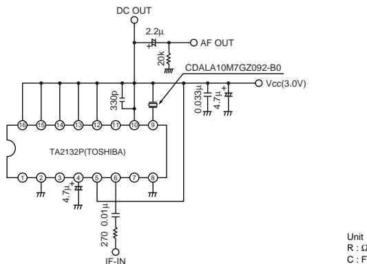
Test Circuit
