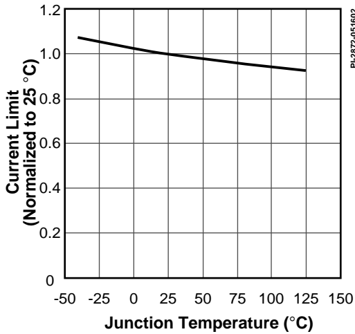
Figure 37. External Current Limit vs. Temperature with R_L = 12\text{ k}\Omega .
