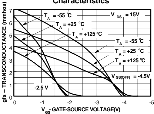
Transconductance Characteristics
