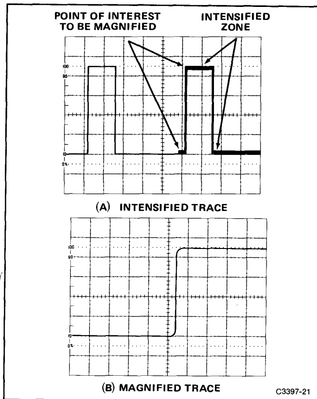
Figure 4-10. Delayed-sweep magnification.
