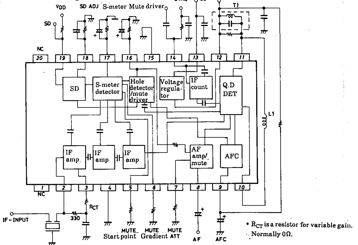
Equivalent Circuit Block Diagram : LA1145M
