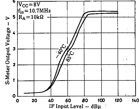
S-Meter Characteristic (Temperature Characteristic)
