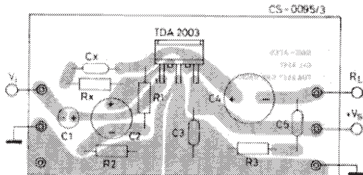
Figure 17. P.C. board and component layout for the circuit of fig. 16 (1 : 1 scale)
