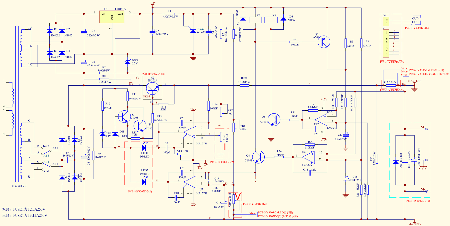
PCB-HY3002D-3 (7) PCB-HY3002D (2)
